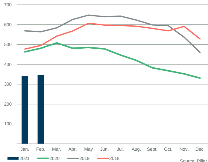
INVENTORY COMPARISON
