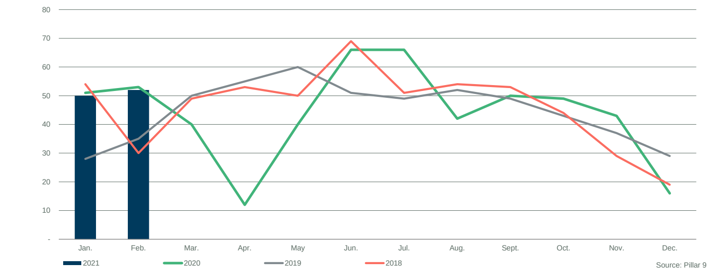
INVENTORY COMPARISON
