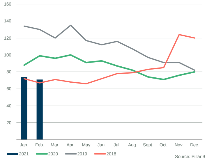
INVENTORY COMPARISON
